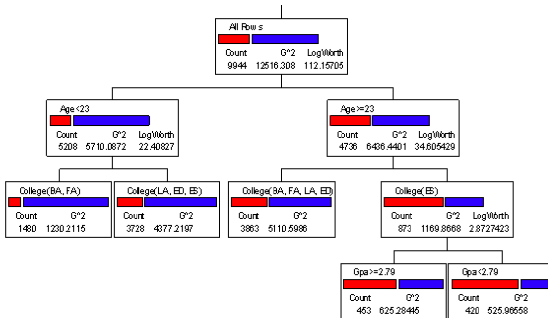
Figure 2. Classification tree.
