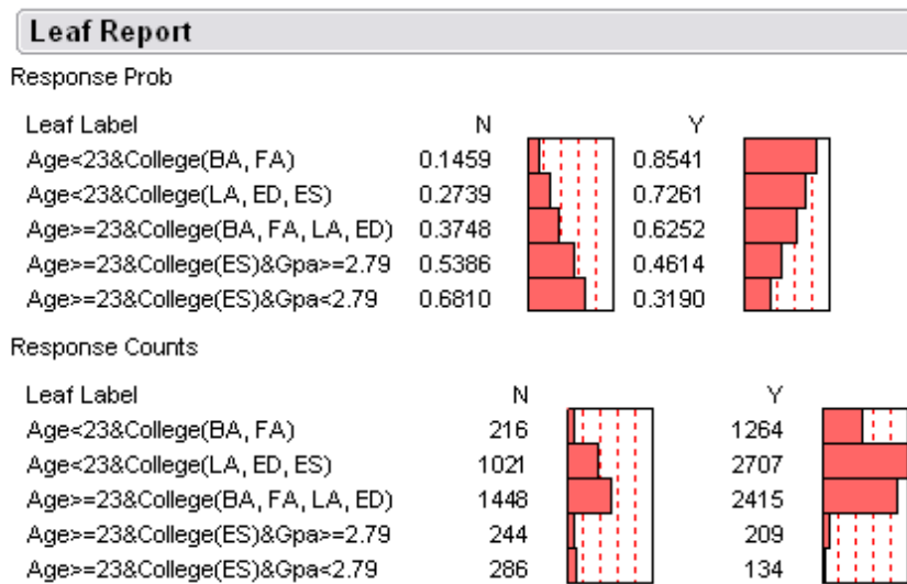
Figure 3. Leaf report.
